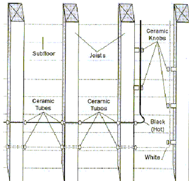
Diagram F1- Typical knob and tube installation
