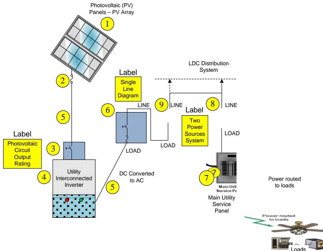
Diagram A: Parallel Meter Connection – microFIT Project
