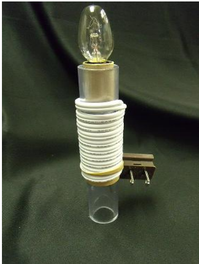
Conductivity Tester with Light Bulb – Opaque plastic
