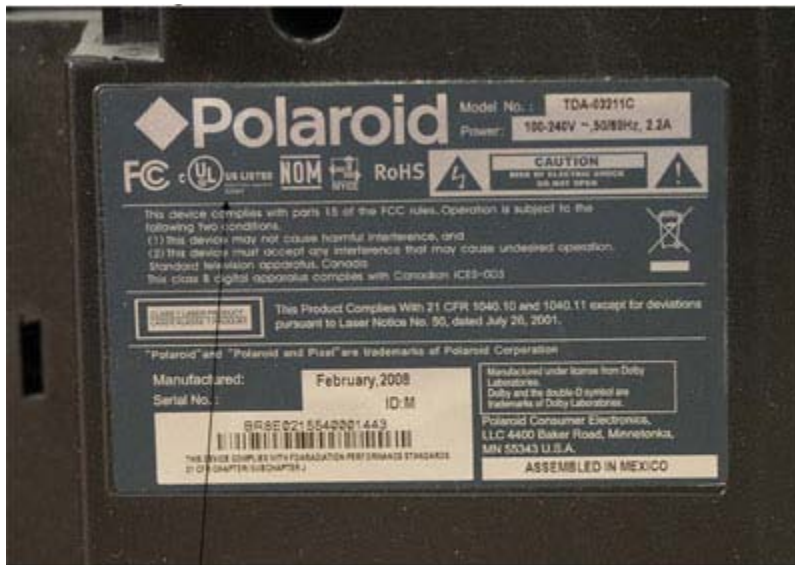
Picture of the Marking Label
